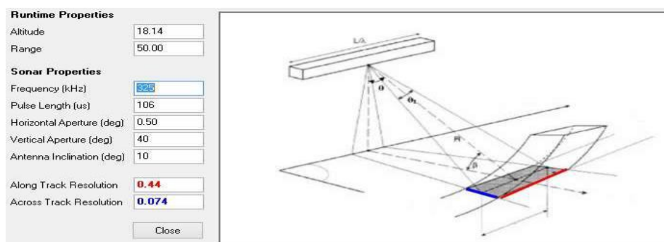
Figure 4. Resolution calculator of SSS survey.
