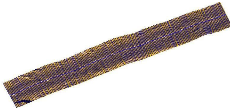
Figure 8. Mosaic and tracklines of SSS imagery.
