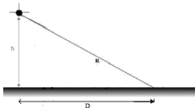
Figure 6. Slant range correction (Blondel 2009).
