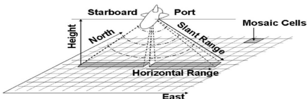
Figure 1. Geometry assumed on SSS.
