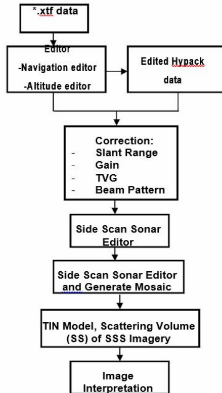
Figure 5. Data flow diagram side scan sonar (SSS).
