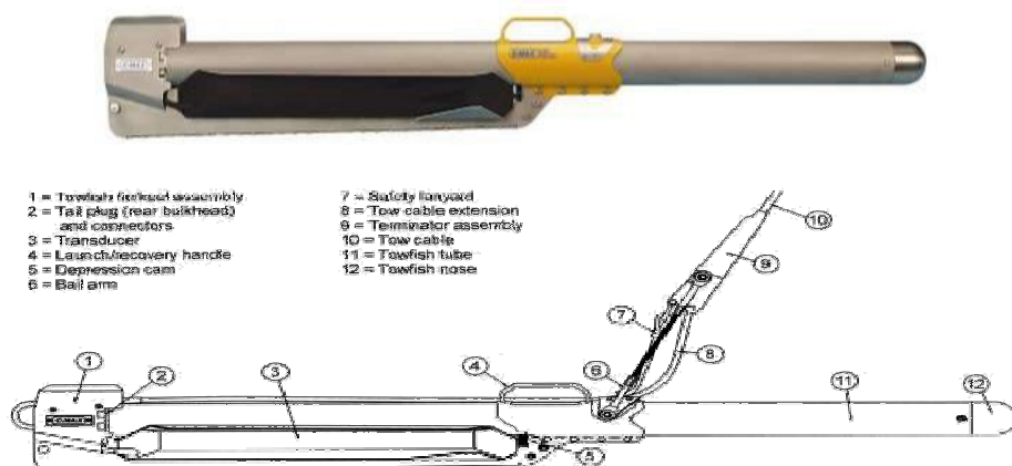
Figure 3. CM2 digital towfish instrument.
