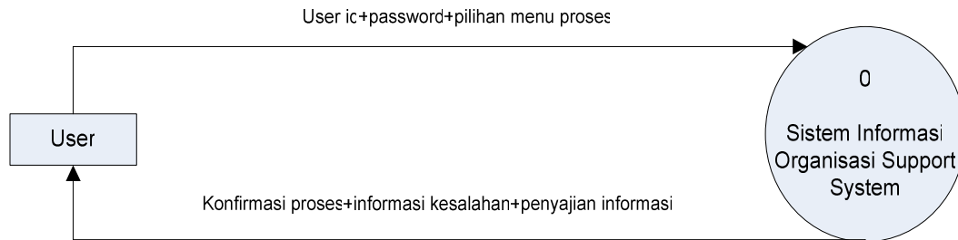
Gambar 3.1.1 Context diagram
