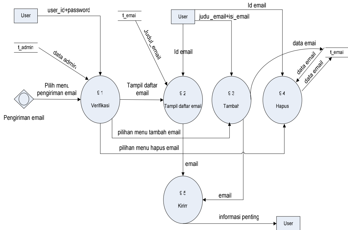
Gambar 3.1.1.6 Proses Email
