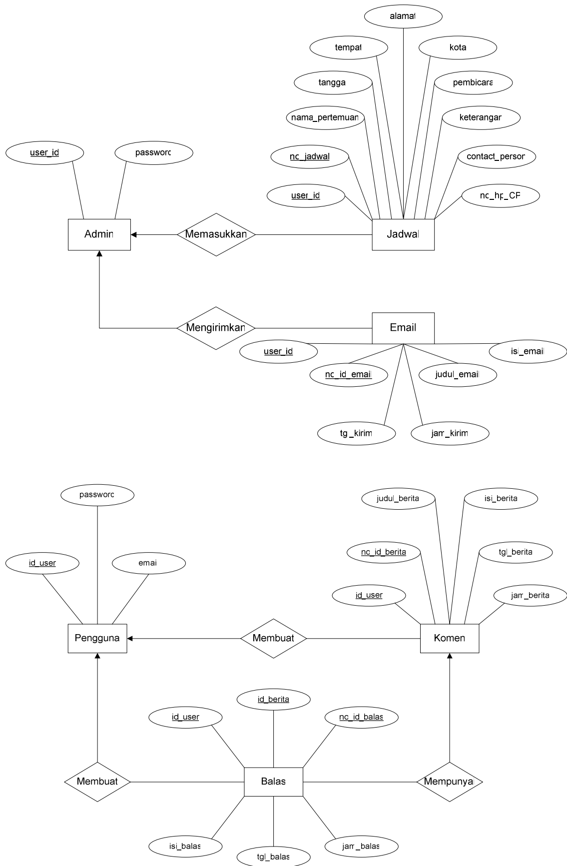
Gambar 3.2.1 E-R diagram
