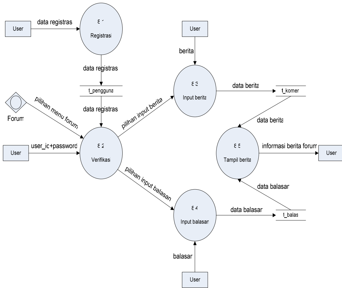
Gambar 3.1.1.5 Proses forum
