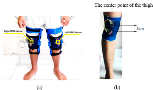
Figure 1. (a) The IMU sensor placement, (b) the distance of the IMU to each knee joint.
