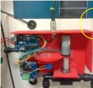
Gambar 6 Wiring DCS to Servo
