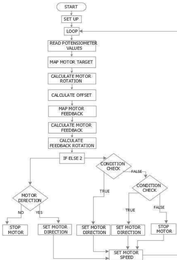
Gambar 5 Flowchart Sistem
