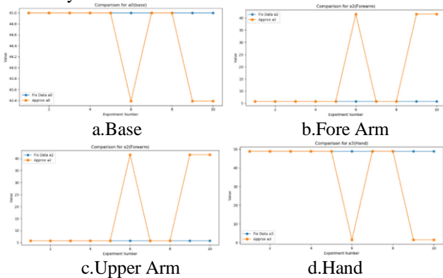
Figure 8. Angle graph during object capture
