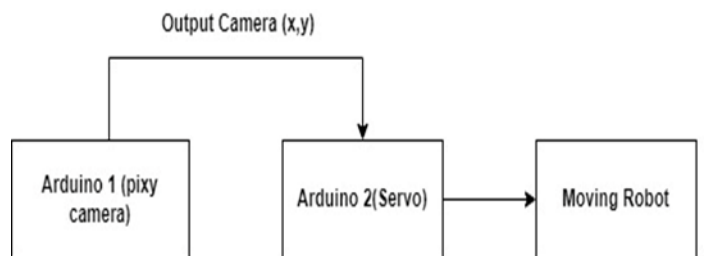
Figure 2. Visual Servoing Hardware Block Diagram
