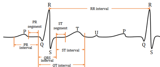
Fig 2. Characteristics waveform of P, QRS dan T [16]
