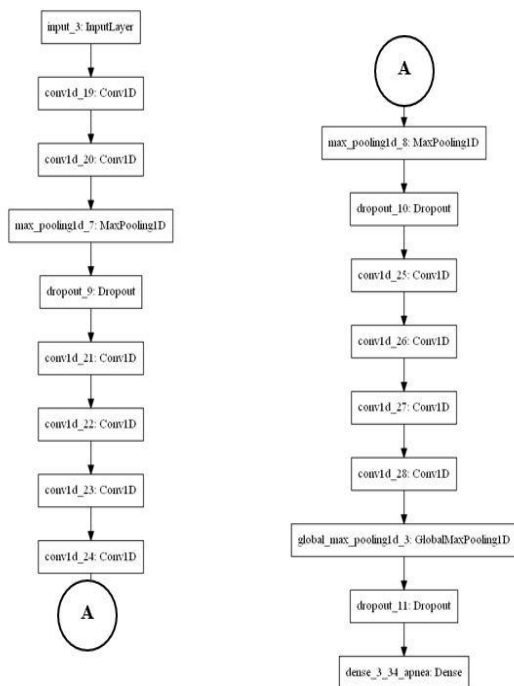
Fig 4. 1D-CNN architecture on 10 second dataset
