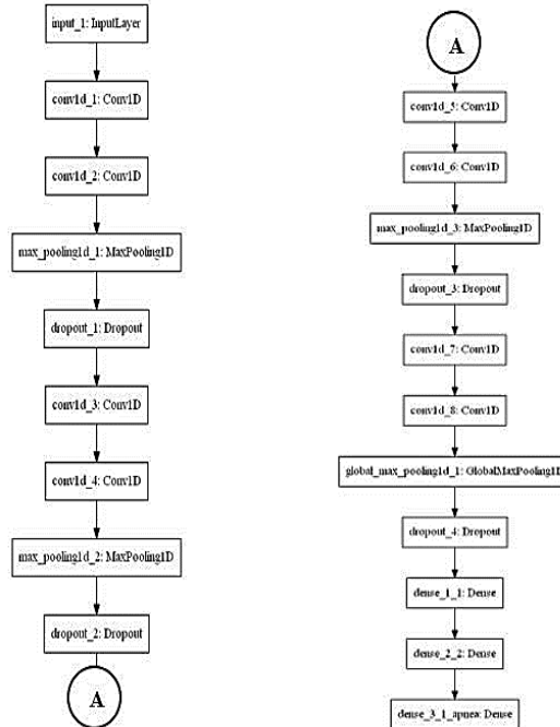
Fig 5. CNN architecture on 20 second dataset
