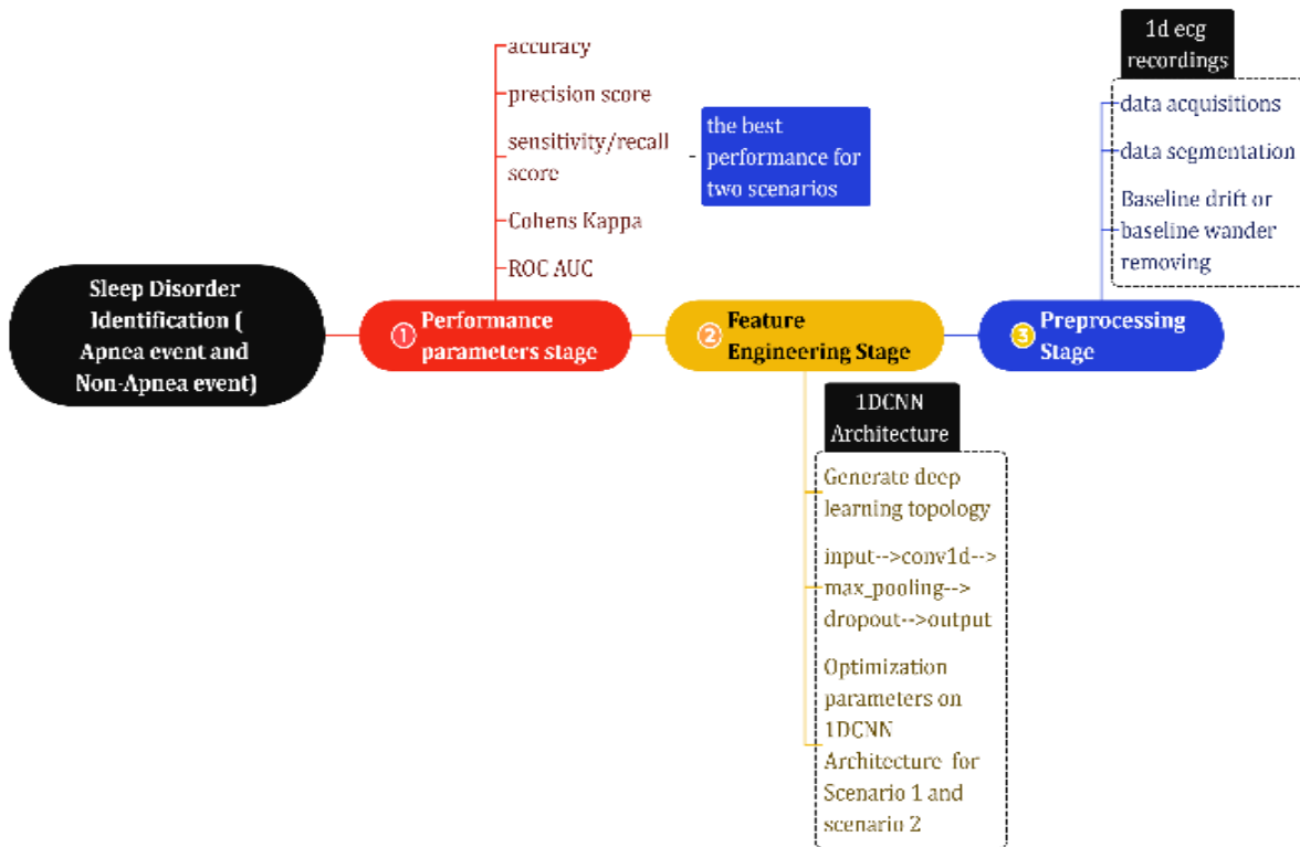
Fig 3. Deep learning framework for identification sleep disorder.
