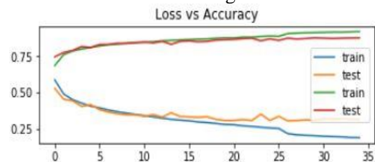
Fig 6. Relationship between accuracy and error performance.
