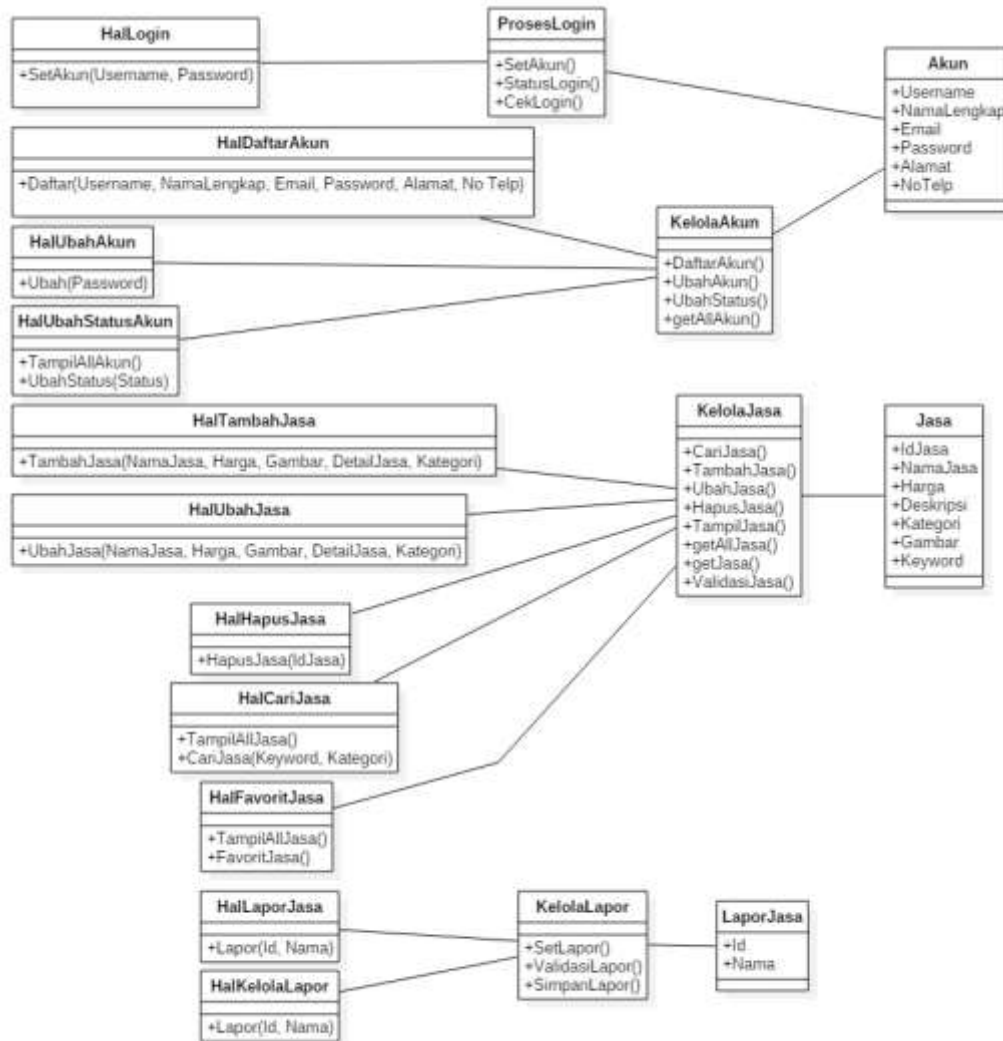
Gambar 3. 13 Class Diagram
