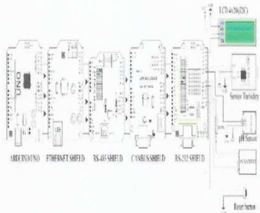
Gambar 5 Wiring Electrical
