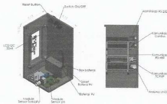
Gambar 6 Design Mekanikal
