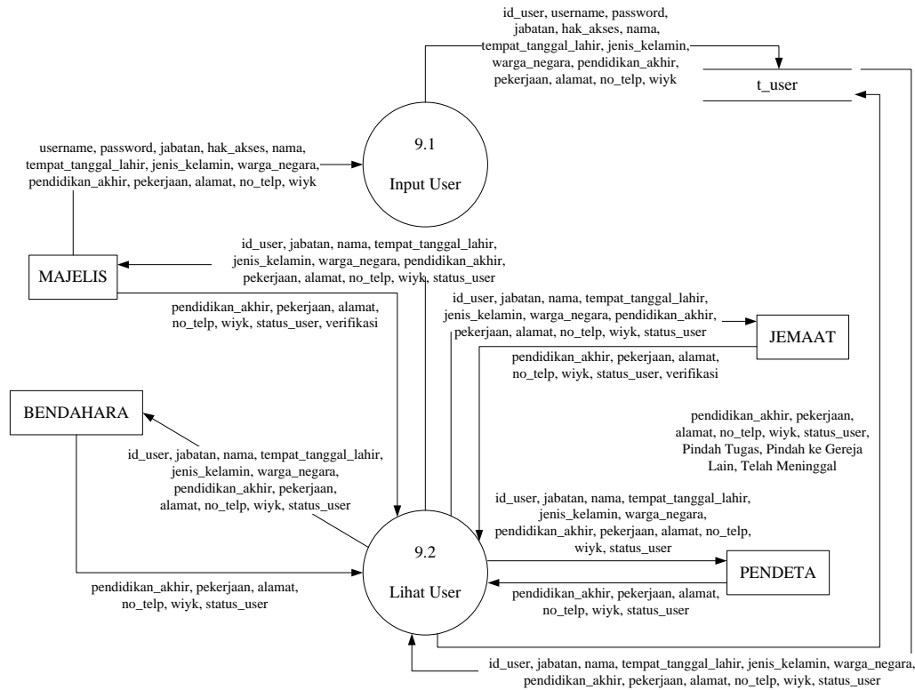
Gambar III-6.3.8 DFD Level 2 Proses 9 User
