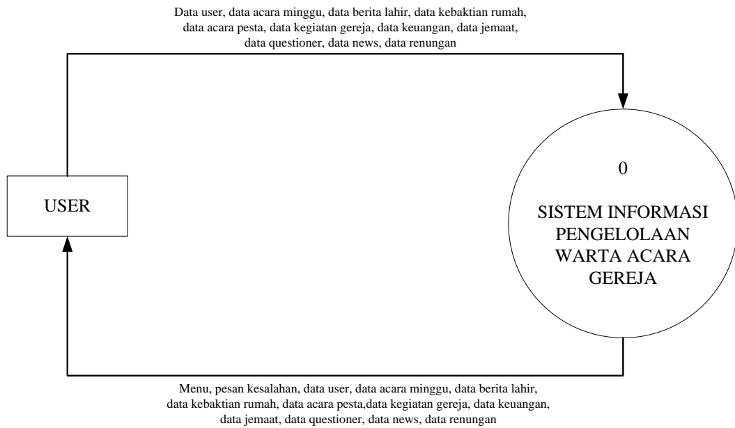
Gambar III-6.1 Context Diagram
