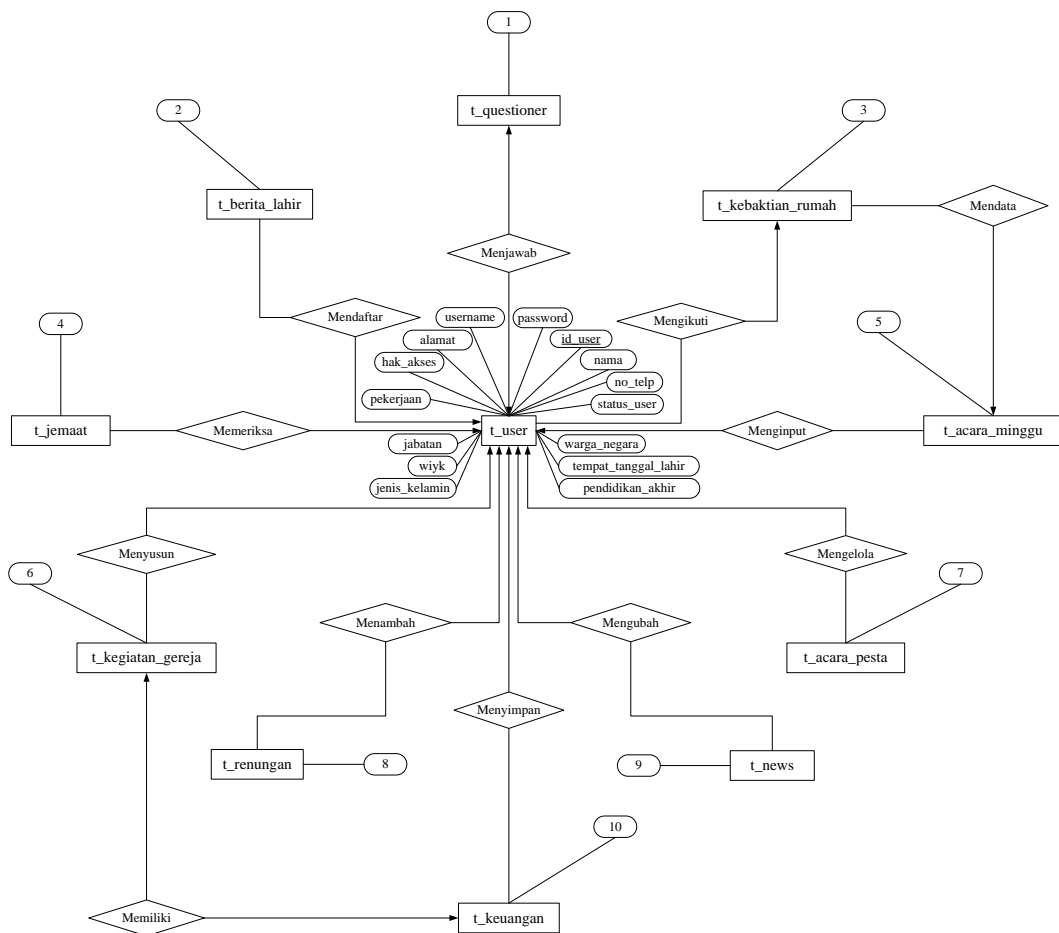
Gambar III-7.1 E-R Diagram
