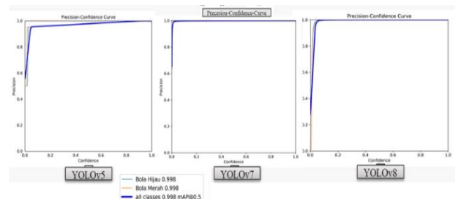
Fig. 6. Precision - Confidence Curve
