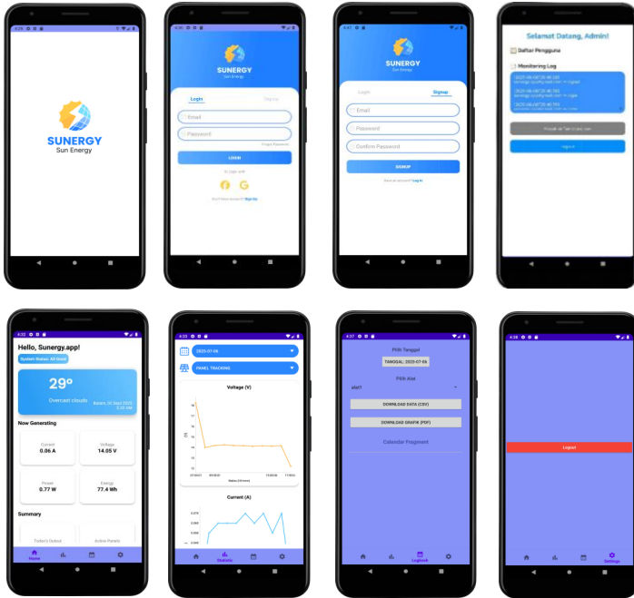
Gambar 23. Tampilan User Interface Android Studio
