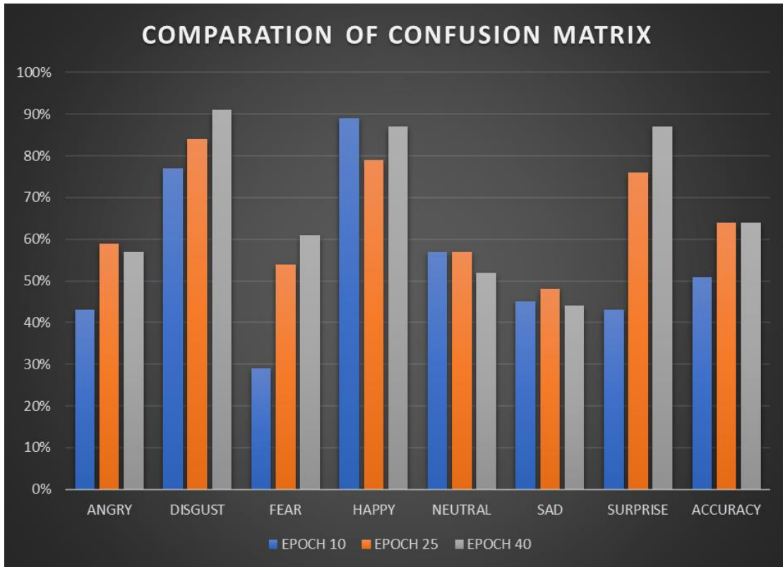
FIGURE 14. Comparison Of Epoch Result
