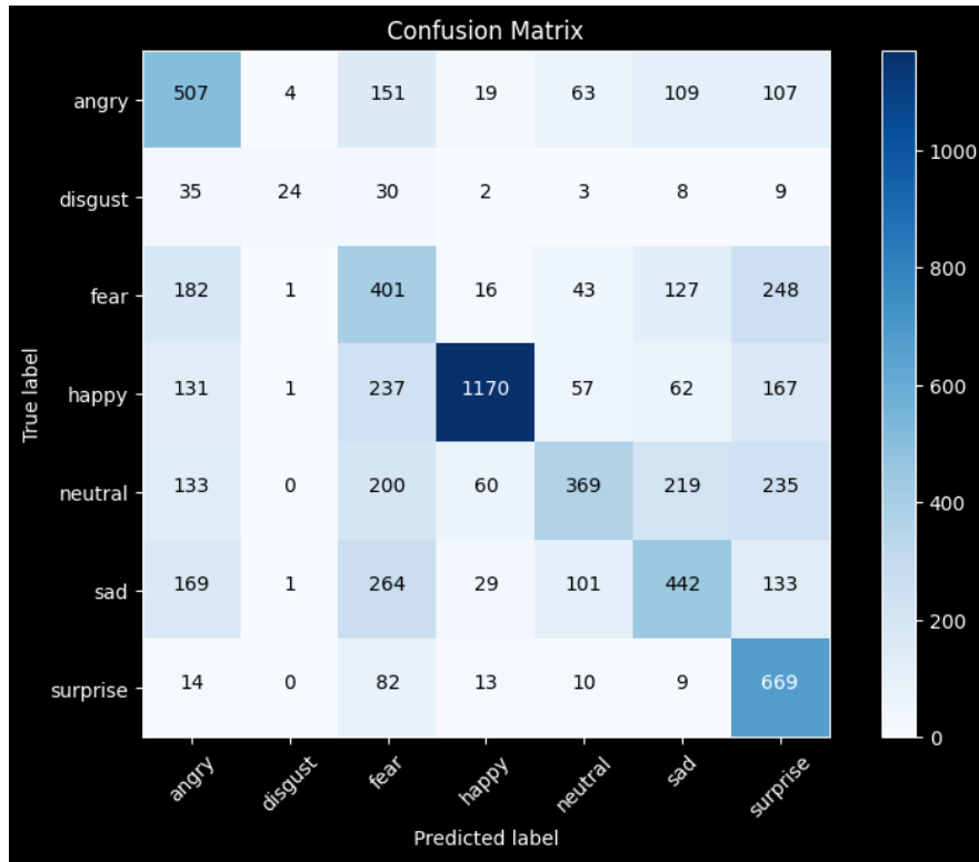
FIGURE 8. 10 Epoch Confusion Matrix
