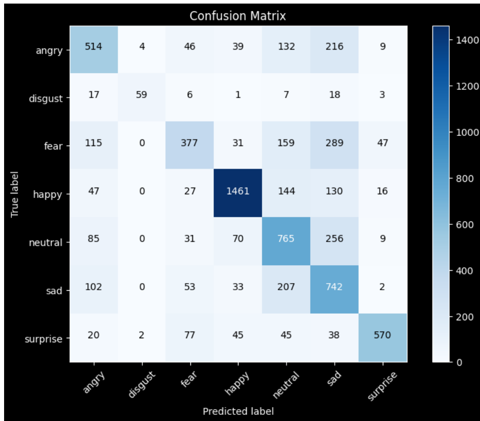
FIGURE 12. 40 Epoch Confusion Matrix
