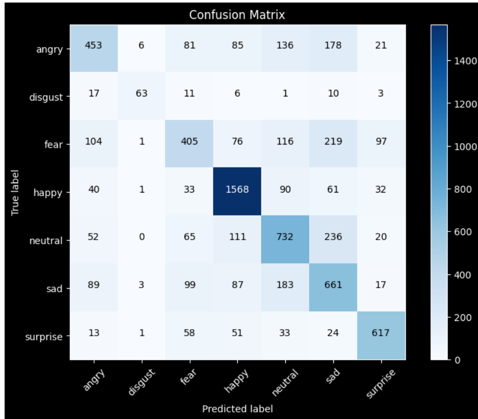
FIGURE 10. 25 Epoch Confusion Matrix
