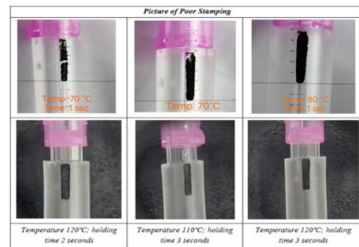
Image 4. Summary of test results for determining temperature and holding time
