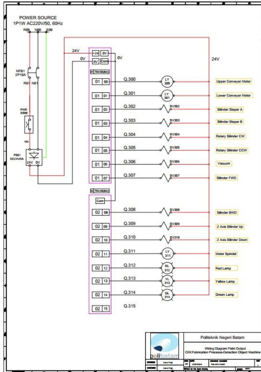
Gambar 37. Wiring diagram field output-1
