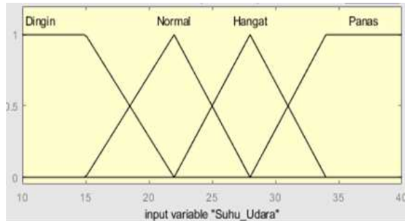
Gambar 5: Membership function input suhu udara
