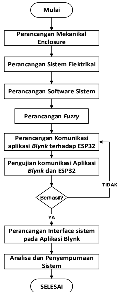
Gambar 1: Flowchart perancangan
