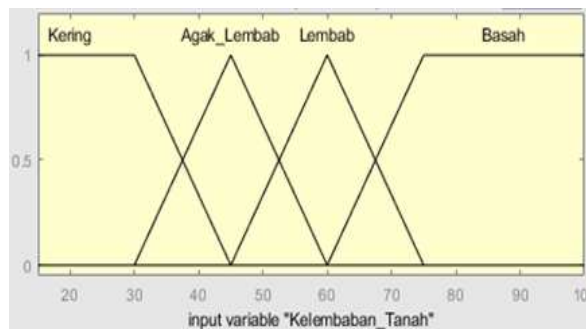
Gambar 6: Membership function input kelembaban tanah
