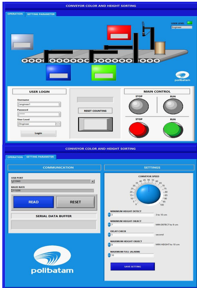
Gambar 11. Hasil Pemrograman HMI User Level Engineer
