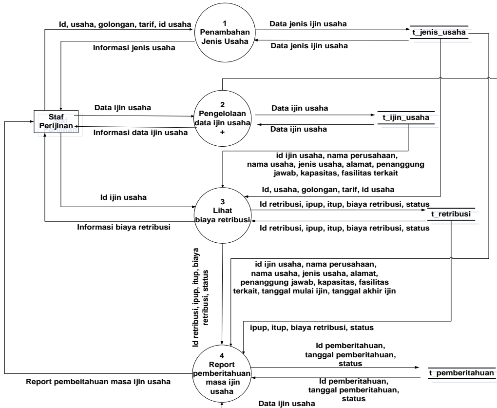
Gambar III.5.2 DFD Level 1
