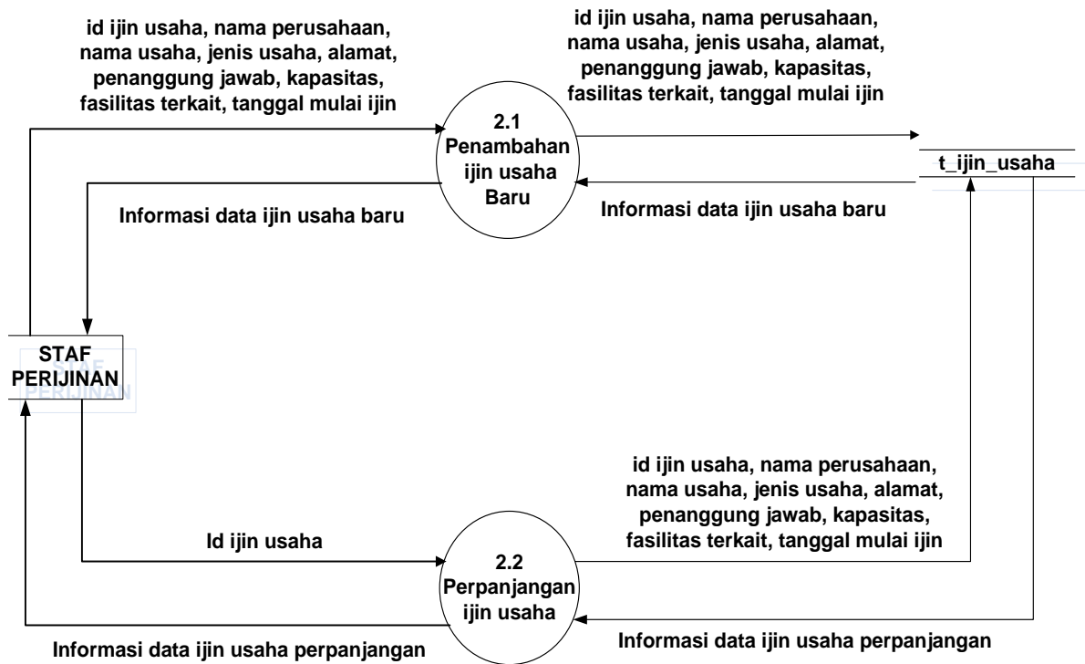
Gambar III.5.3 DFD Level 2 Proses 2
