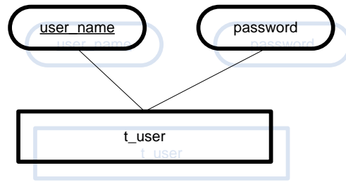
Gambar 3.7 Entitas User
