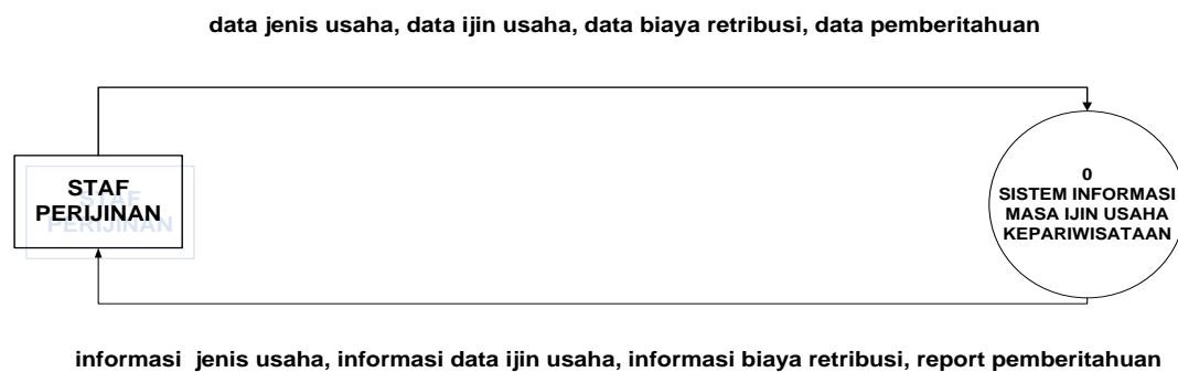
Gambar III.5.1 Context Diagram
