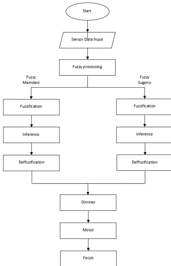
Figure 2. System Flowchart
