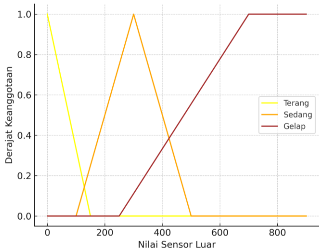
Figure 6. Outdoor Sensor Membership Function Graph
