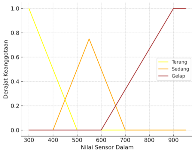
Figure 5. Indoor Sensor Membership Function Graph
