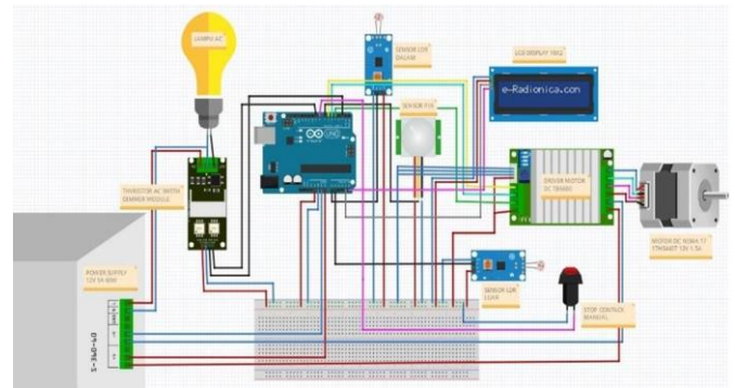
Figure 4. Electrical Design
