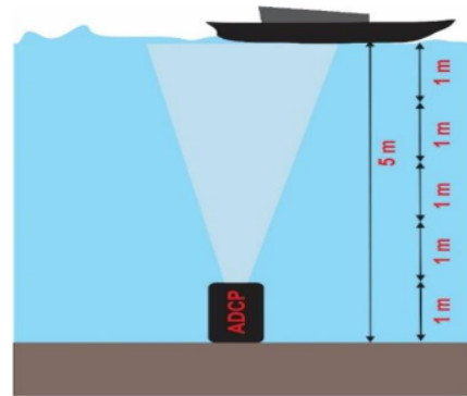
Figure 2 ADCP current data collection scheme.
