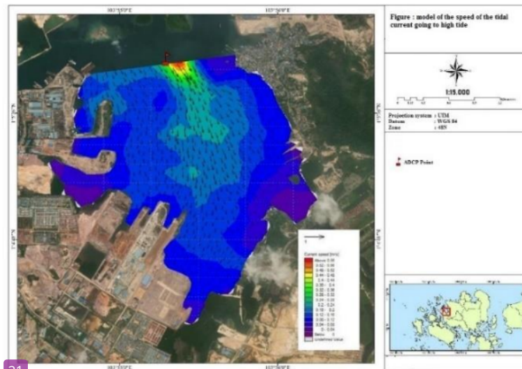
21 Figure 13 Model of the tidal current speed to the tide.
